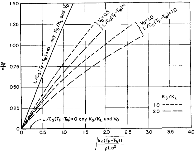
Fig. 4. Effect of thermal diffusivity ratio on the location of freezing front.
